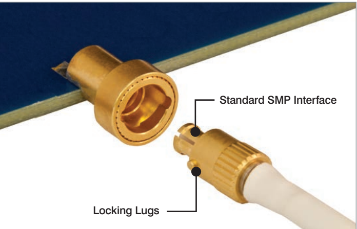
Secure-Lok Mechanism
